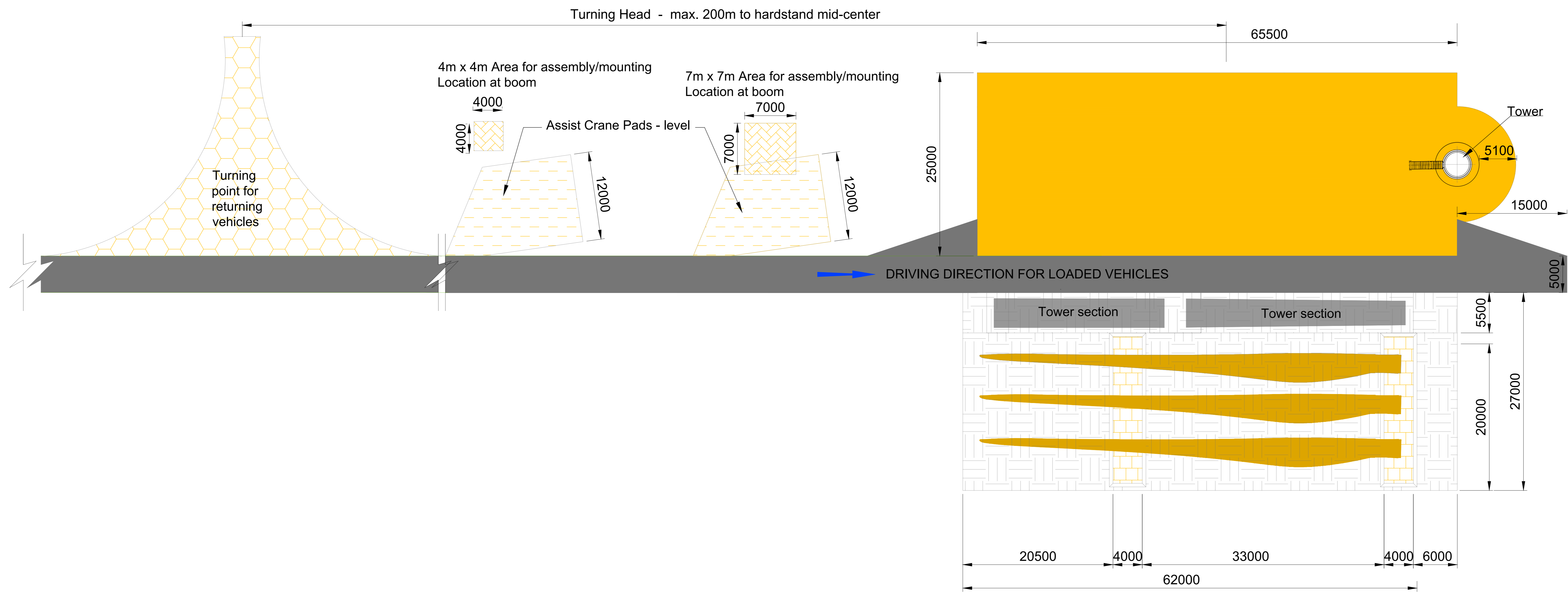
HARDSTAND LAYOUT PLAN ( CONSTRUCTION )
